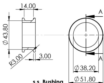
s.s. Bushing P/N 207105
