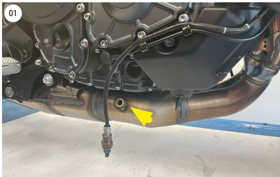
unscrew the sonda lamba / O2 sensor
