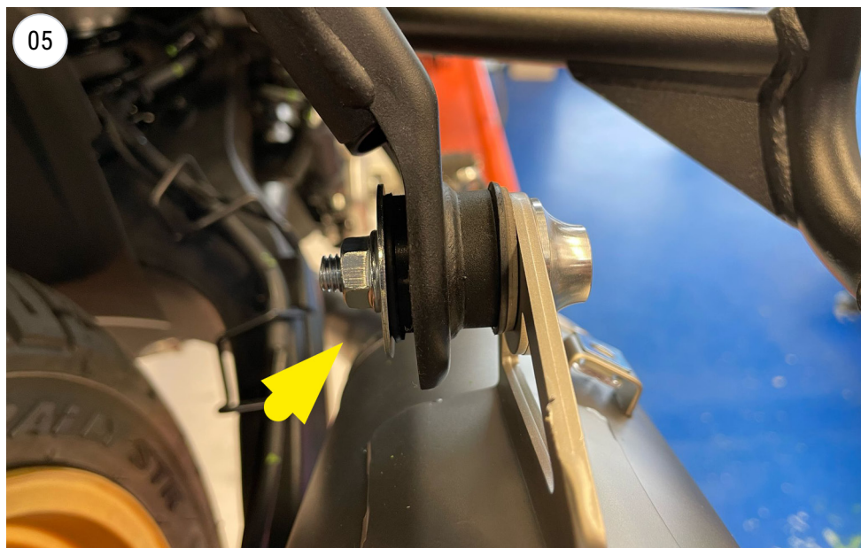
screw stacking
